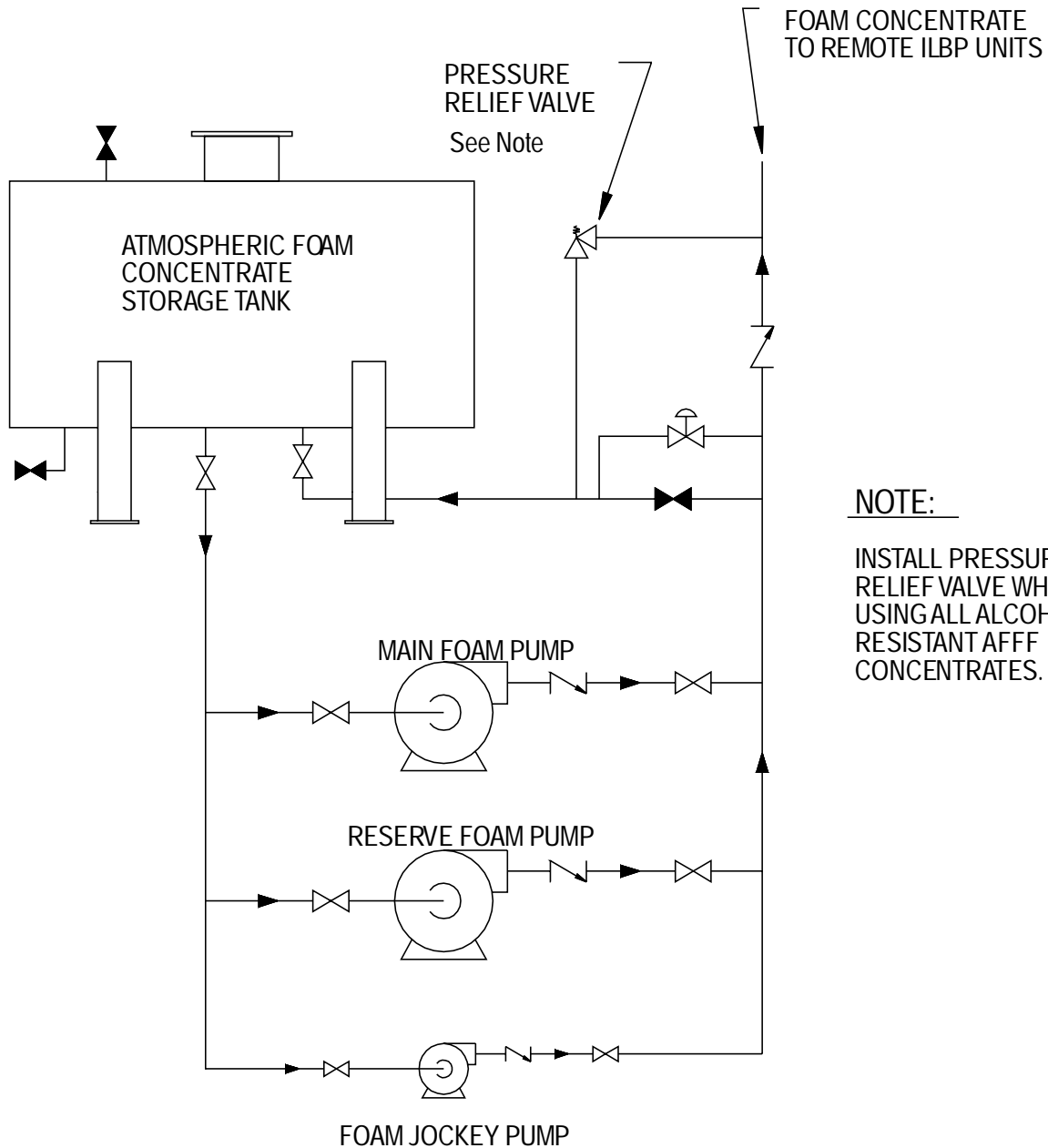
FOAM SYSTEM USING MAIN RESERVE FOAM PUMPS with JOCKEY PUMP TO IN-LINE BALANCED PRESSURE PROPORTIONING UNITS
