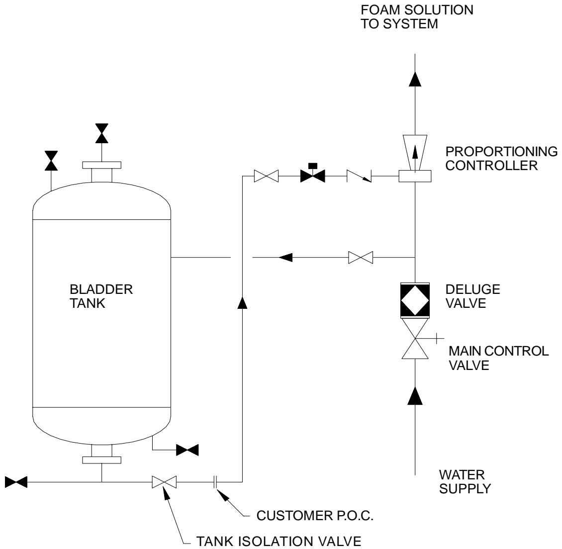
VERTICAL BLADDER TANK with ONE PROPORTIONING CONTROLLER
